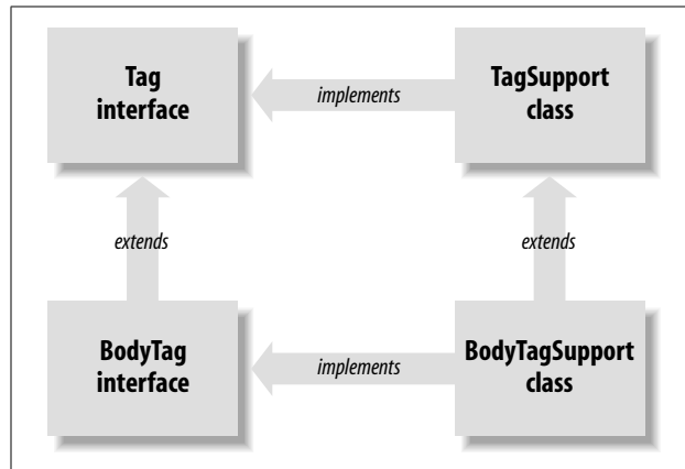
Figure 4. The primary tag-extension interfaces and support classes
